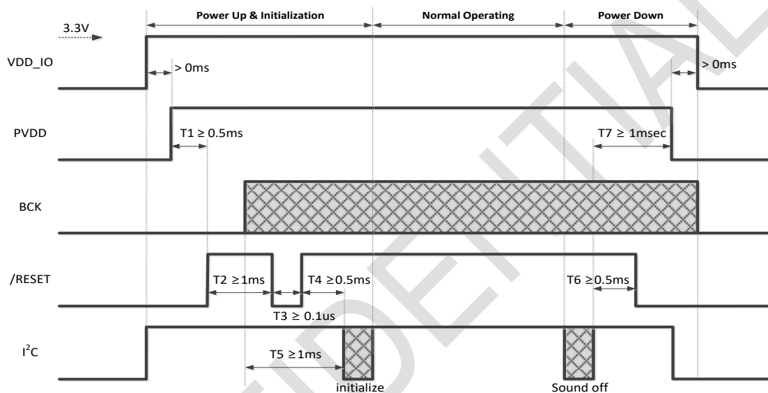
Figure 10. Timing Sequence 1
