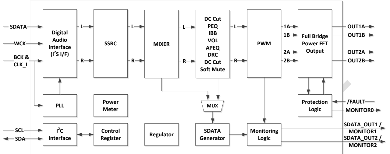
Figure 1. NTP8928 Block Diagram
