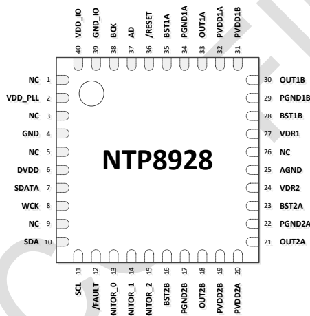
(40 pin QFN 6mm x 6mm Package)
