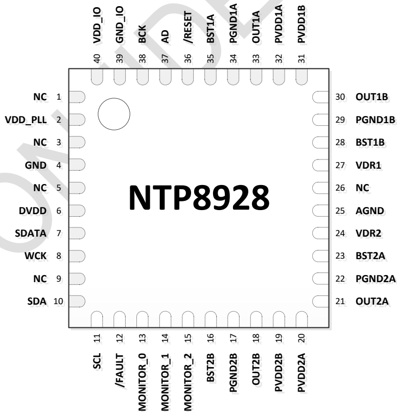
Figure 2. NTP8928 Pin Assignments
