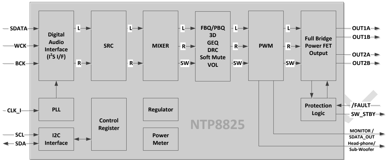
Figure 1. NTP8825 Block Diagram
