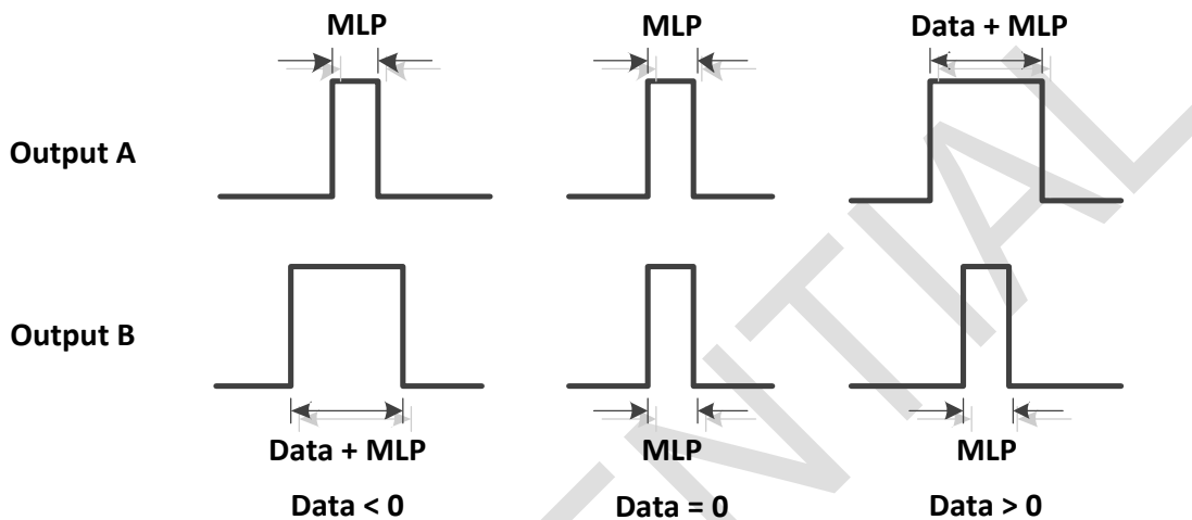
Figure 22. Compensation by MLP
