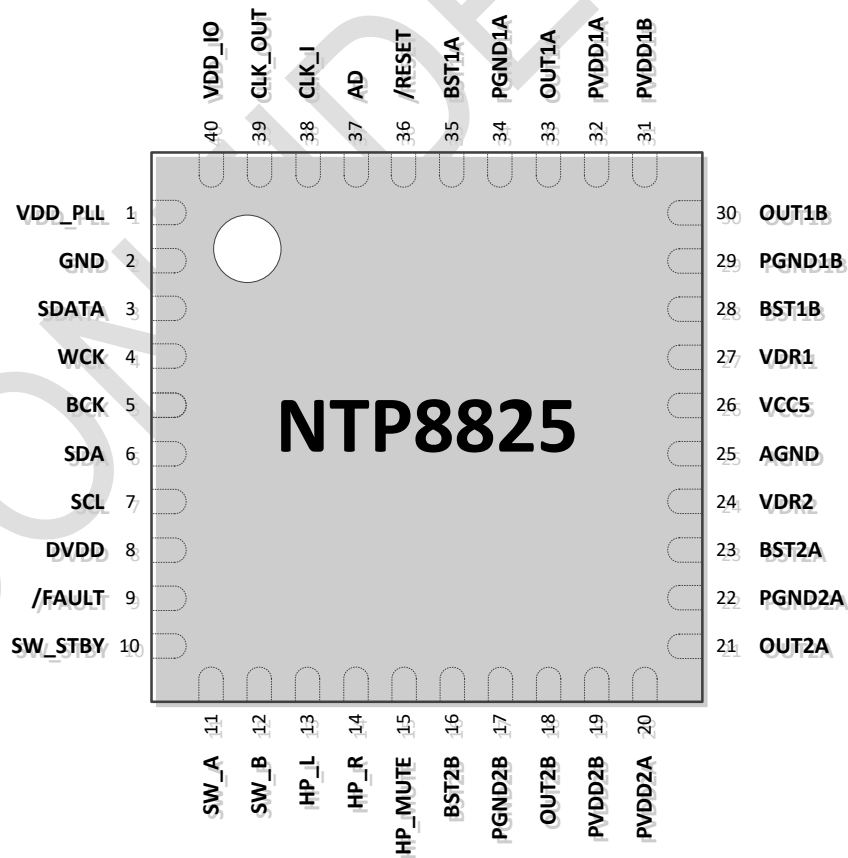
Figure 2. NTP8825 Pin Assignments
