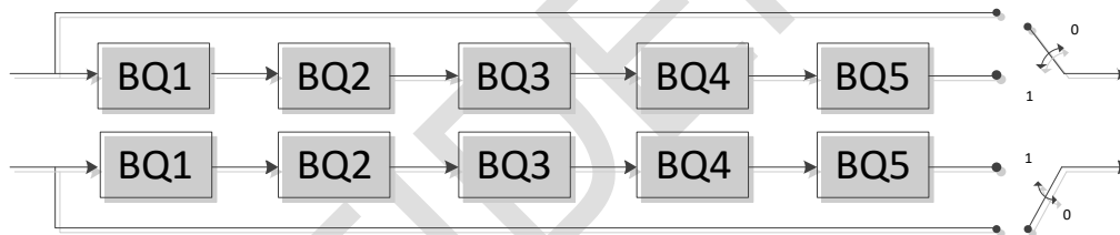
Figure 17. Configurable Graphic Equalizer
