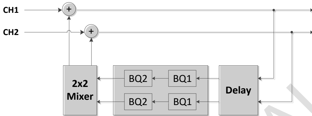
Figure 16. 3D Surround Structure
