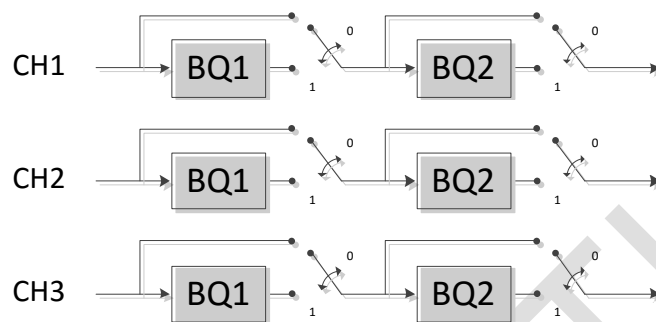
Figure 14. Pre Bi-Quad Filter Structure
