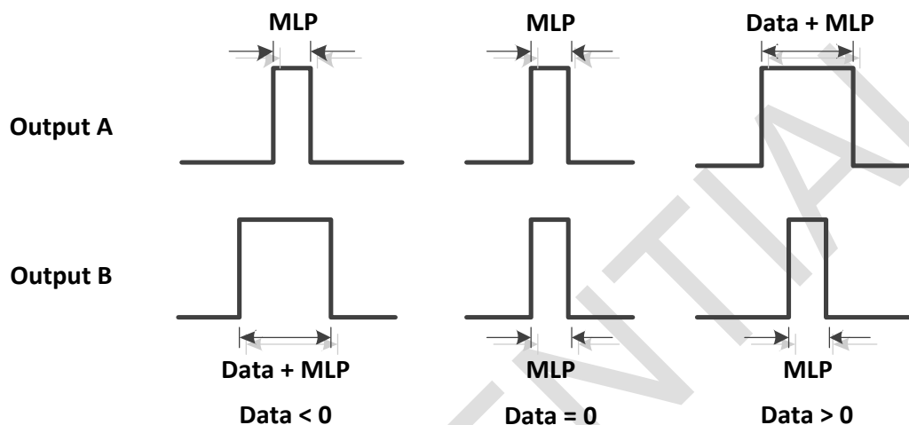
Figure 22. Compensation by MLP
