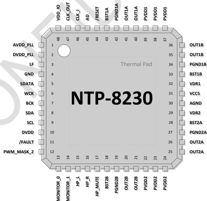
Figure 2. NTP8230G Pin Assignments
