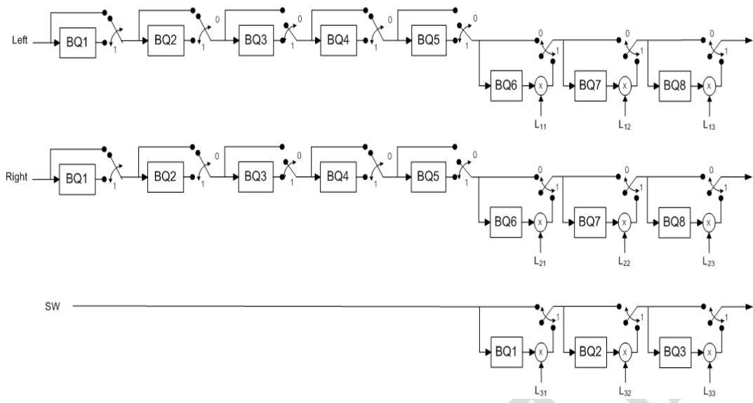
Figure 18. Post Bi-Quad Filter Structure
