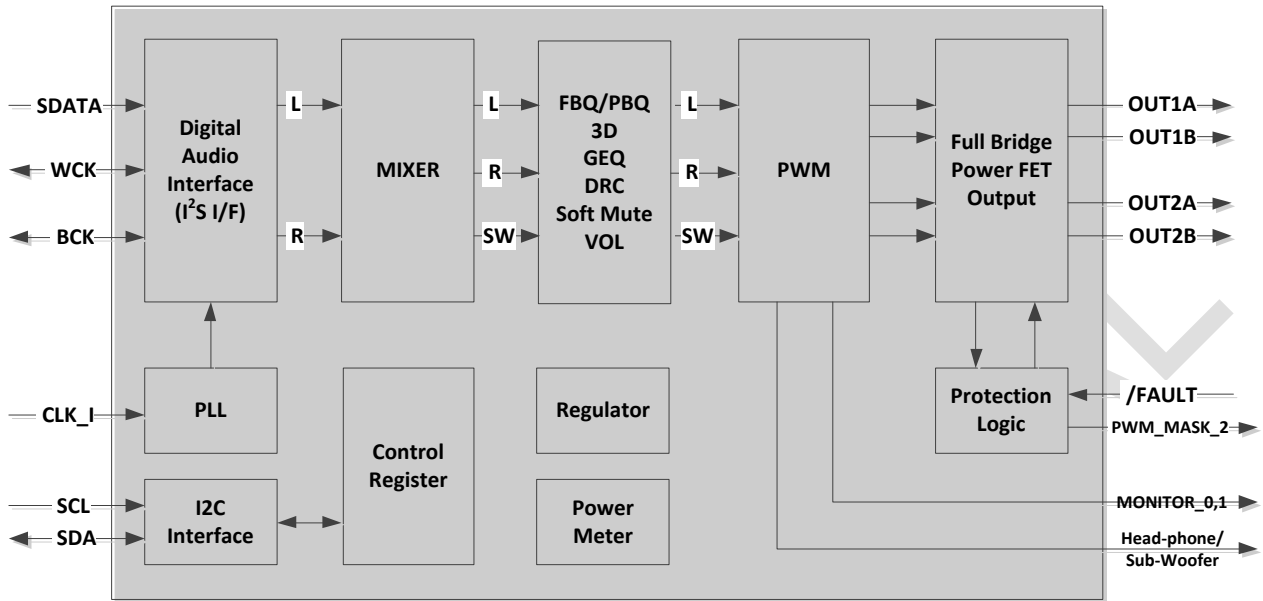
Figure 1. NTP8230G Block Diagram
