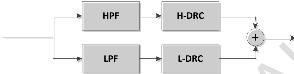
Figure 19. Block Diagram of Dynamic Range Control
