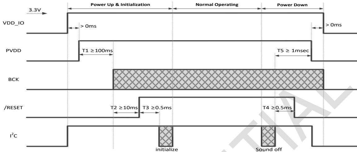
Figure 11. Timing Sequence 2
