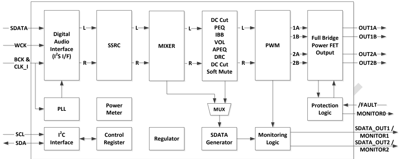
Figure 1. NTP8918 Block Diagram
