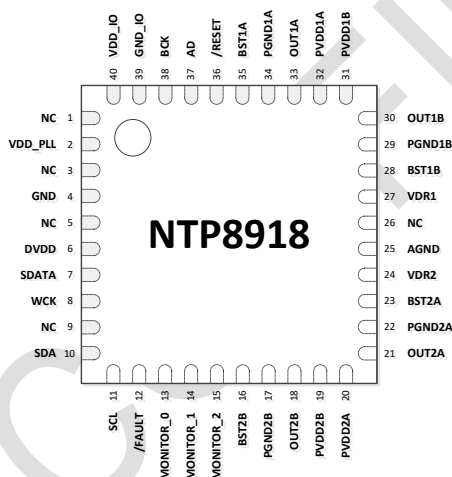
(40 pin QFN 6mm x 6mm Package)
