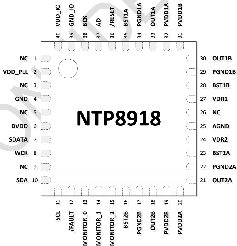
Figure 2. NTP8918 Pin Assignments
